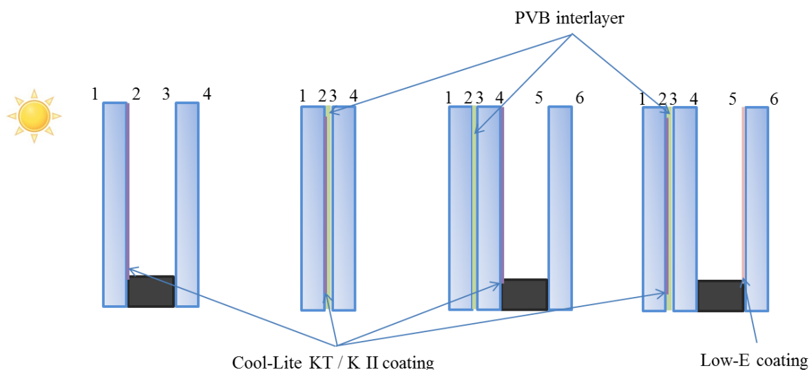
Figure 2: Possible configurations of use of Cool-Lite KT / KII. In all cases, the coating must be edge deleted.
